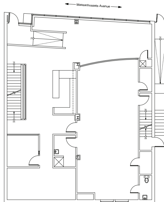
First Floor (Ground Floor)
